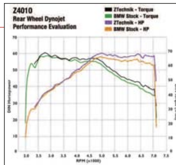
Z4010 Dyno Chart
