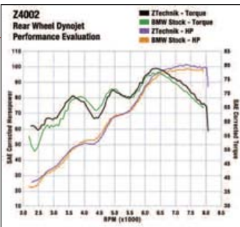
Z4002 Dyno Chart
