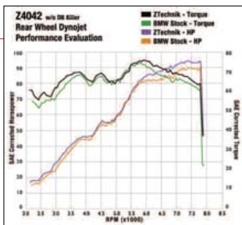
Z4042 Dyno Chart
