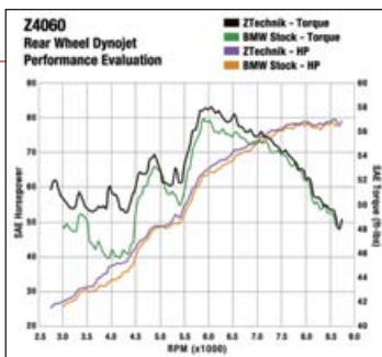
Z4060 Dyno Chart
